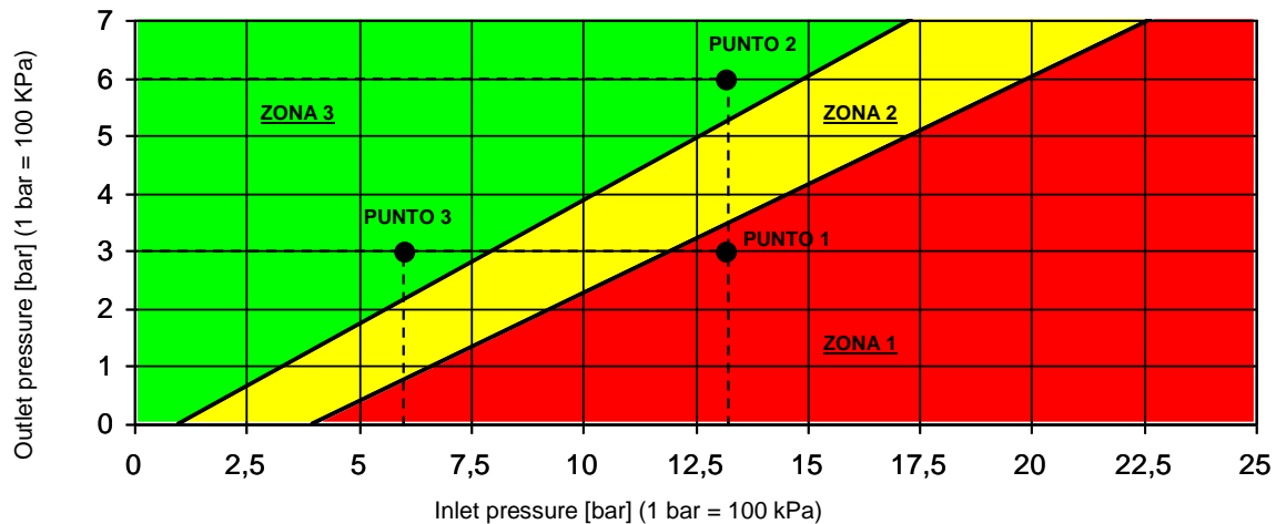
CAVITATION DIAGRAM *
